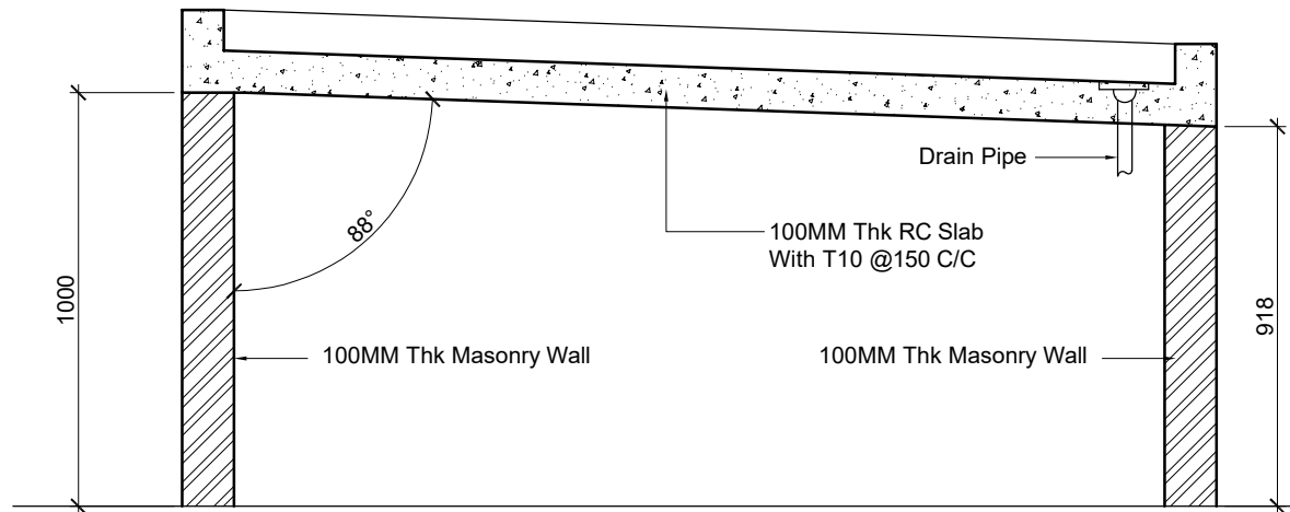
Section
